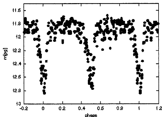
Photographic light curve of NSV 1012. The dots refer to sliding means (N=3) of the individual estimates
